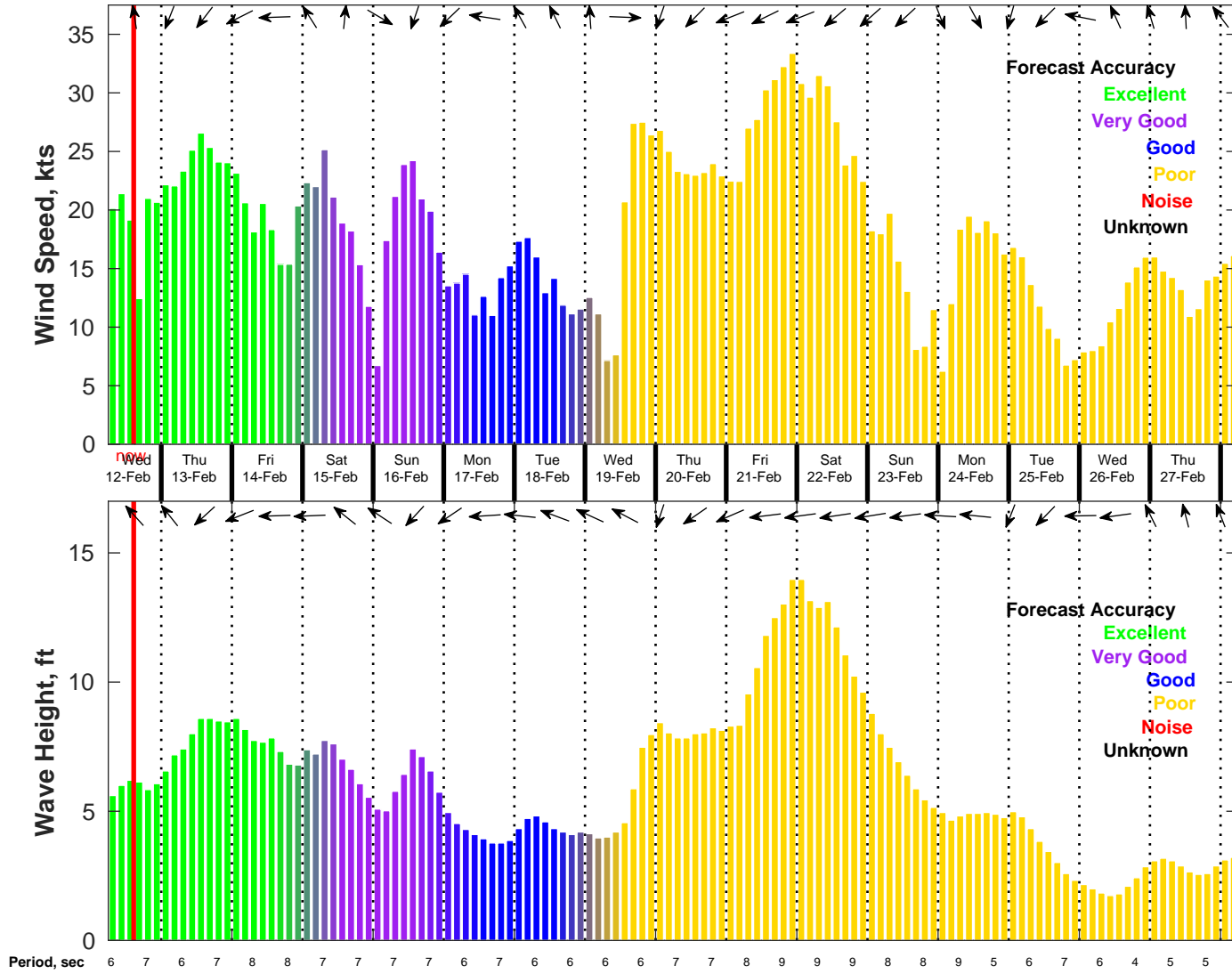
Wind & Wave Forecast for NDBC 42019 from 12-Feb-2025 06:00:00 to 28-Feb-2025 06:00:00
