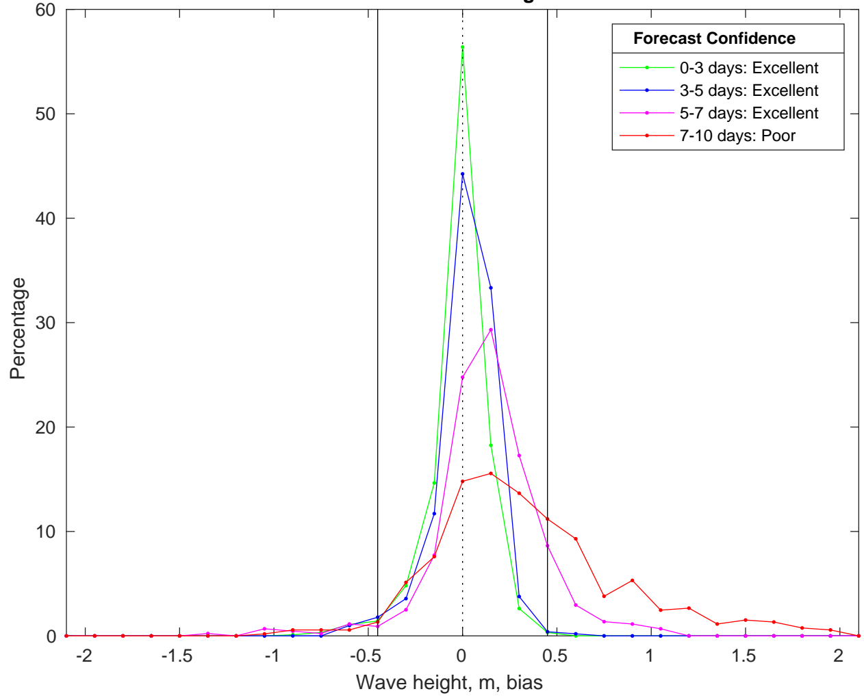
NDBC 42020 vs CMEMS Waves Bias Histogram: 12-Feb-2025
