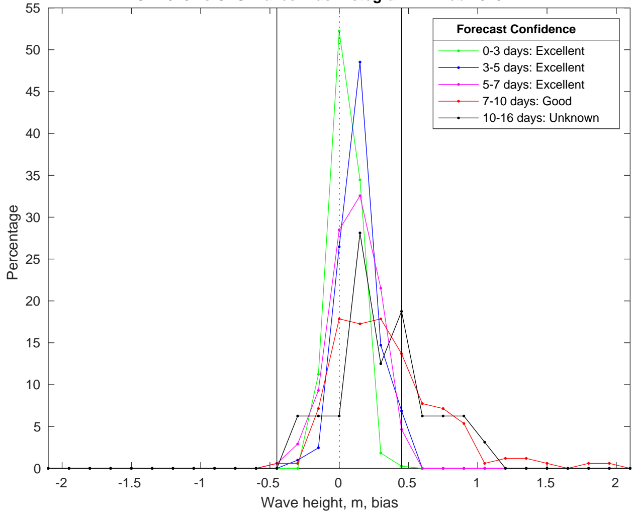
NDBC 42020 vs GFS Waves Bias Histogram: 12-Feb-2025
