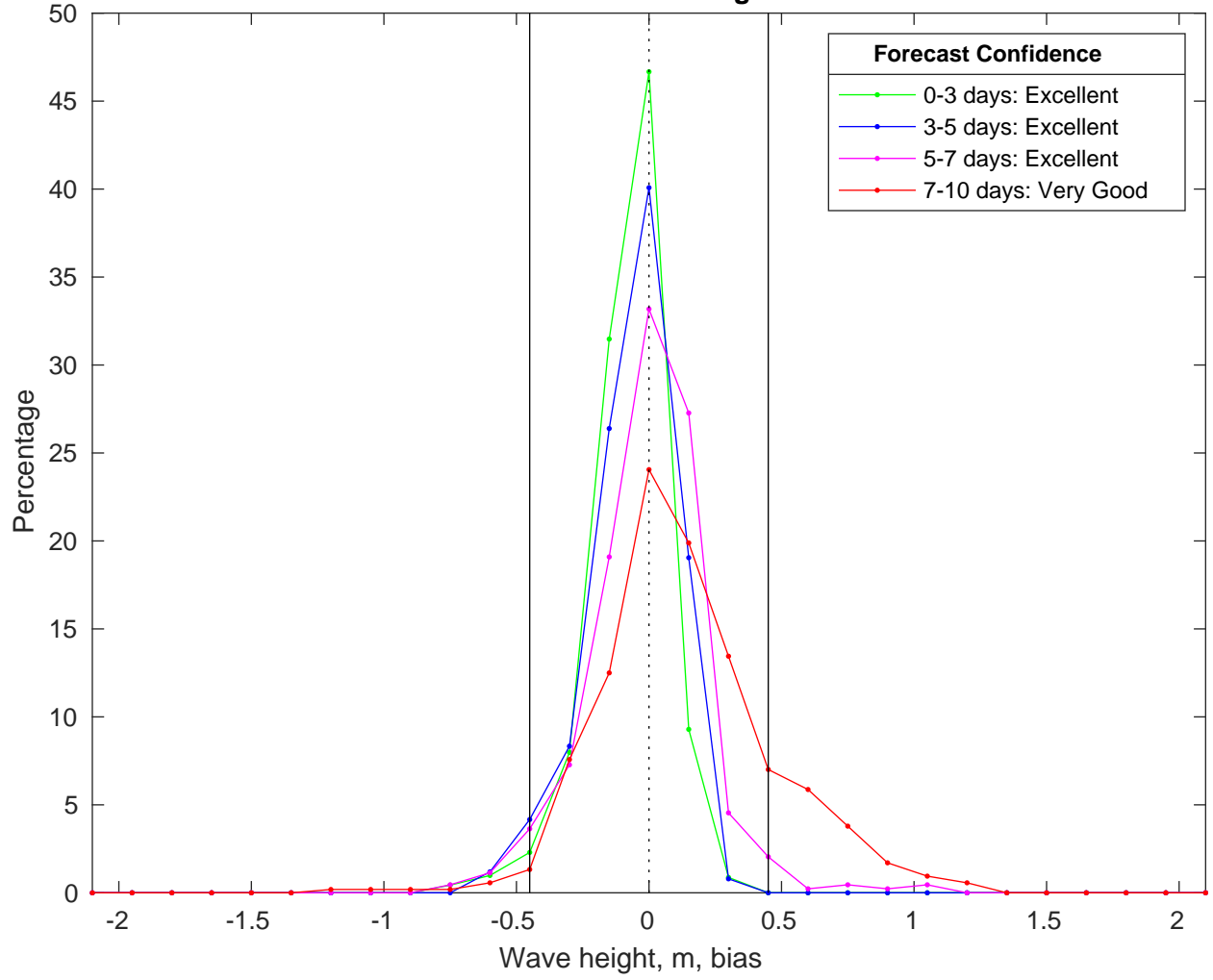
NDBC 42035 vs CMEMS Waves Bias Histogram: 12-Feb-2025
