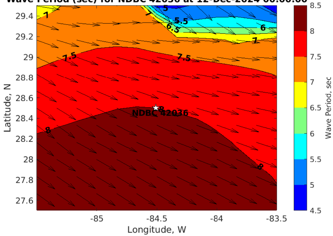
Wave Period (sec) for NDBC 42036 at 12-Dec-2024 00:00:00
