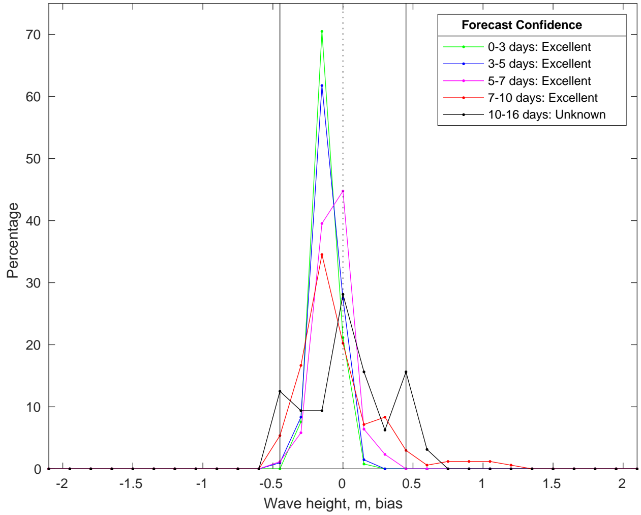
NDBC 42036 vs GFS Waves Bias Histogram: 12-Feb-2025
