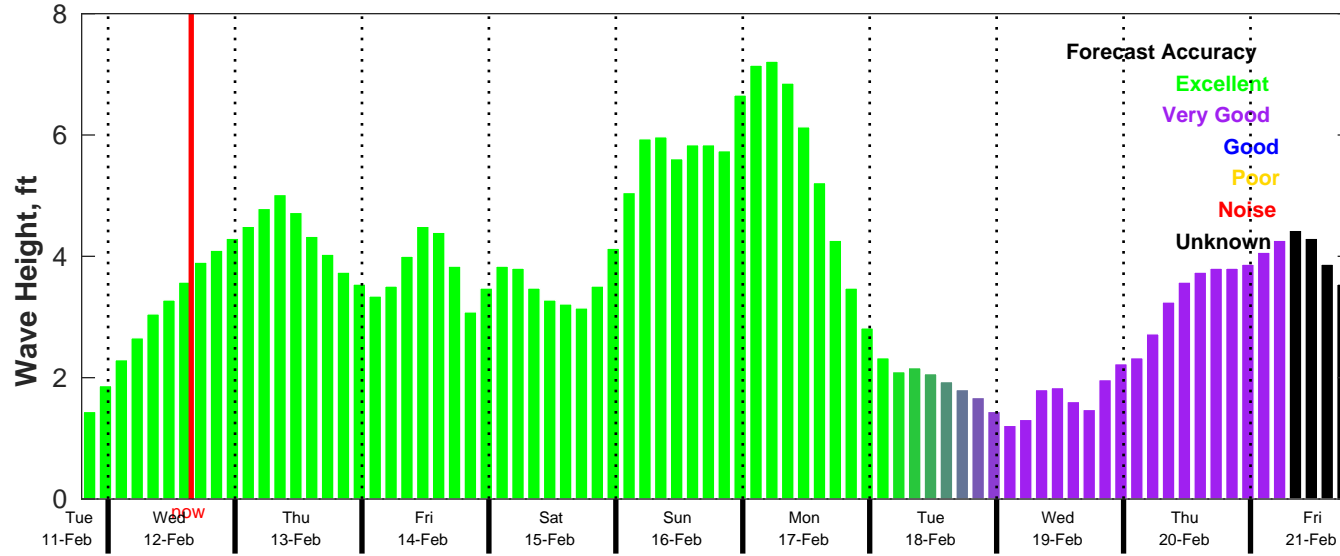
CMEMS Wave Forecast for NDBC 42036 from 11-Feb-2025 19:00:00 to 21-Feb-2025 19:00:00
