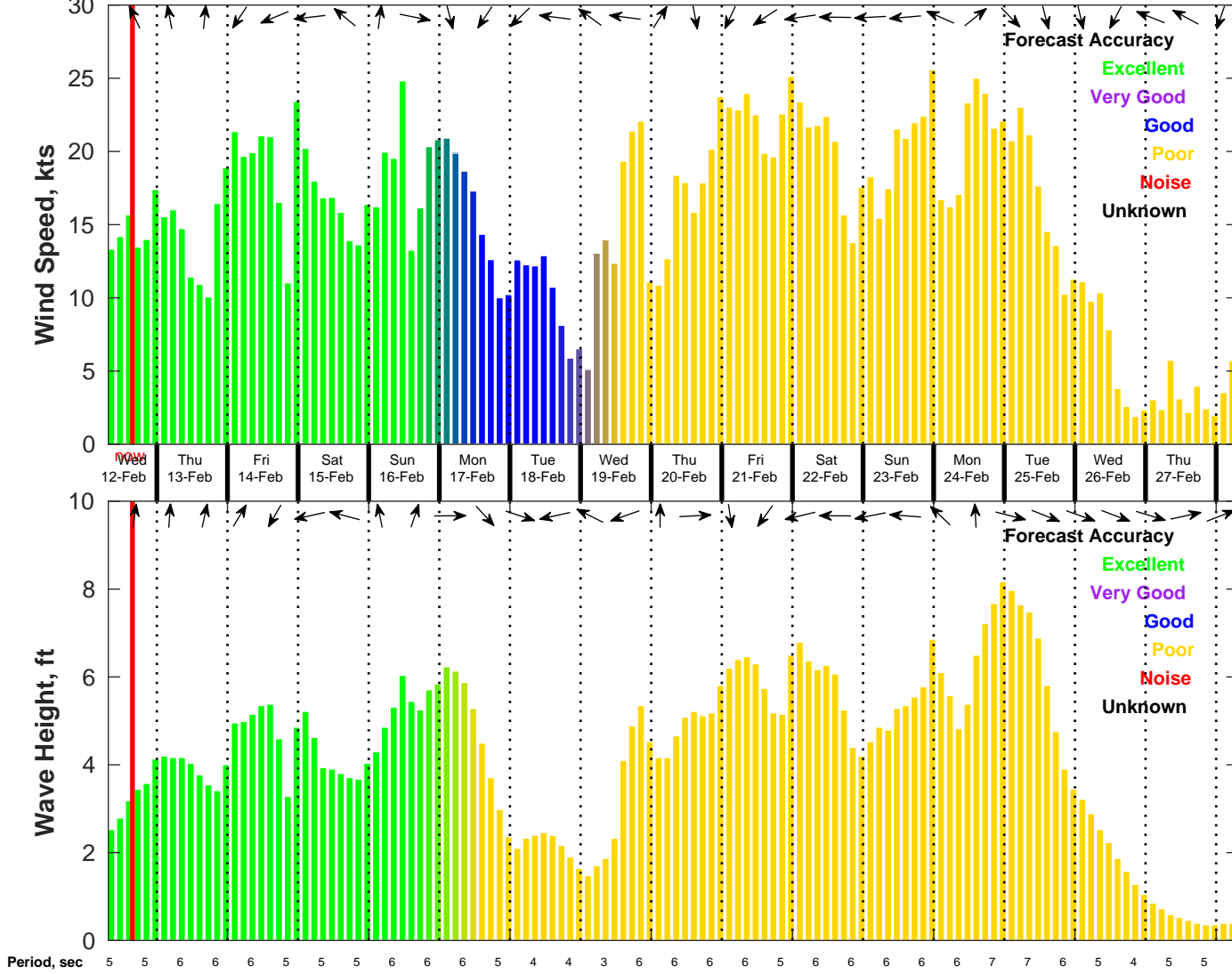
Wind & Wave Forecast for NDBC 42036 from 12-Feb-2025 07:00:00 to 28-Feb-2025 07:00:00
