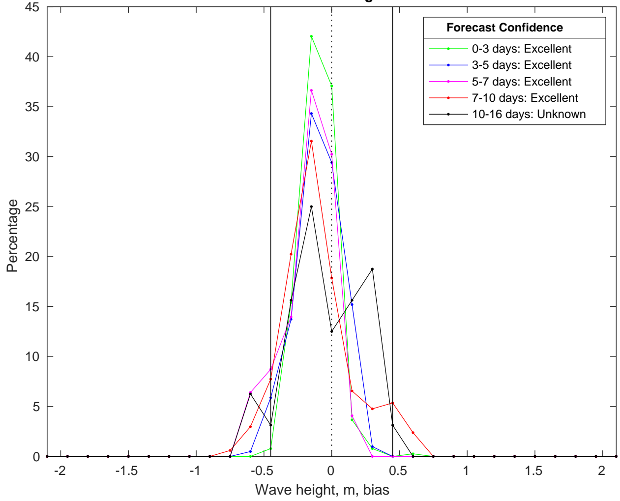
NDBC 42040 vs GFS Waves Bias Histogram: 12-Feb-2025
