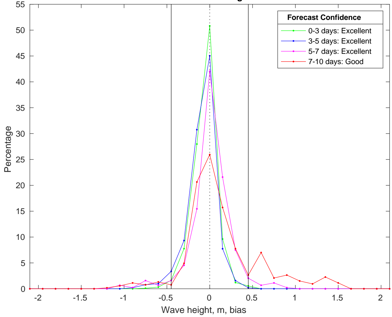
NDBC 42084 vs CMEMS Waves Bias Histogram: 12-Feb-2025
