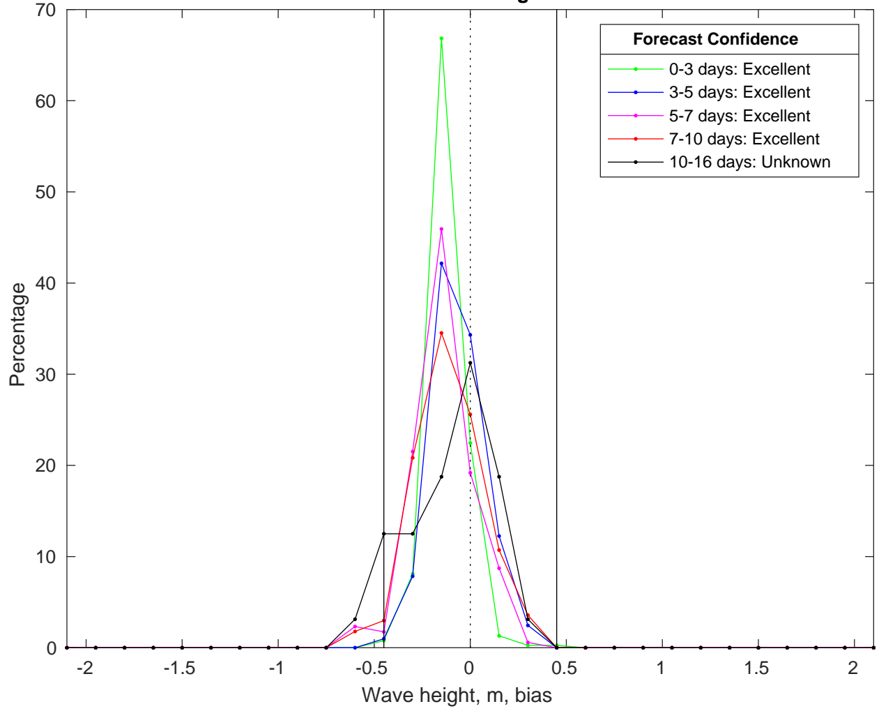
NDBC 42084 vs GFS Waves Bias Histogram: 12-Feb-2025
