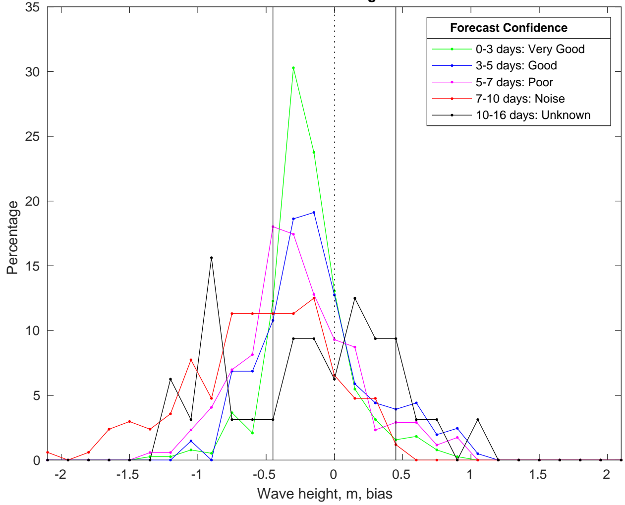
NDBC 46011 vs GFS Waves Bias Histogram: 12-Feb-2025
