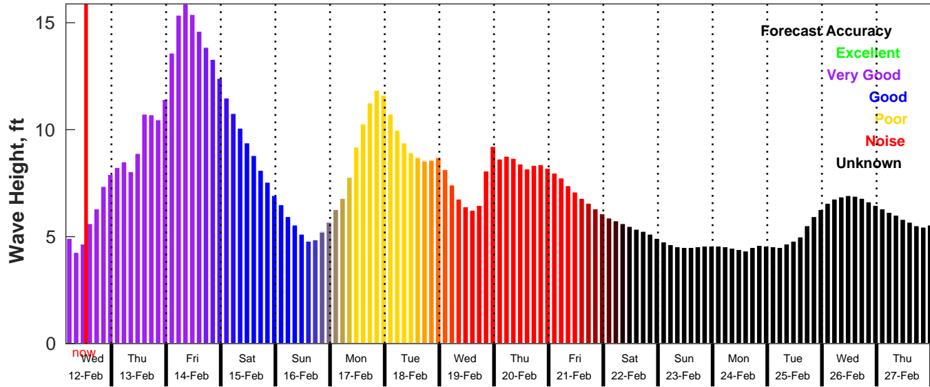
GFS Wave Forecast for NDBC 46011 from 12-Feb-2025 04:00:00 to 28-Feb-2025 04:00:00
