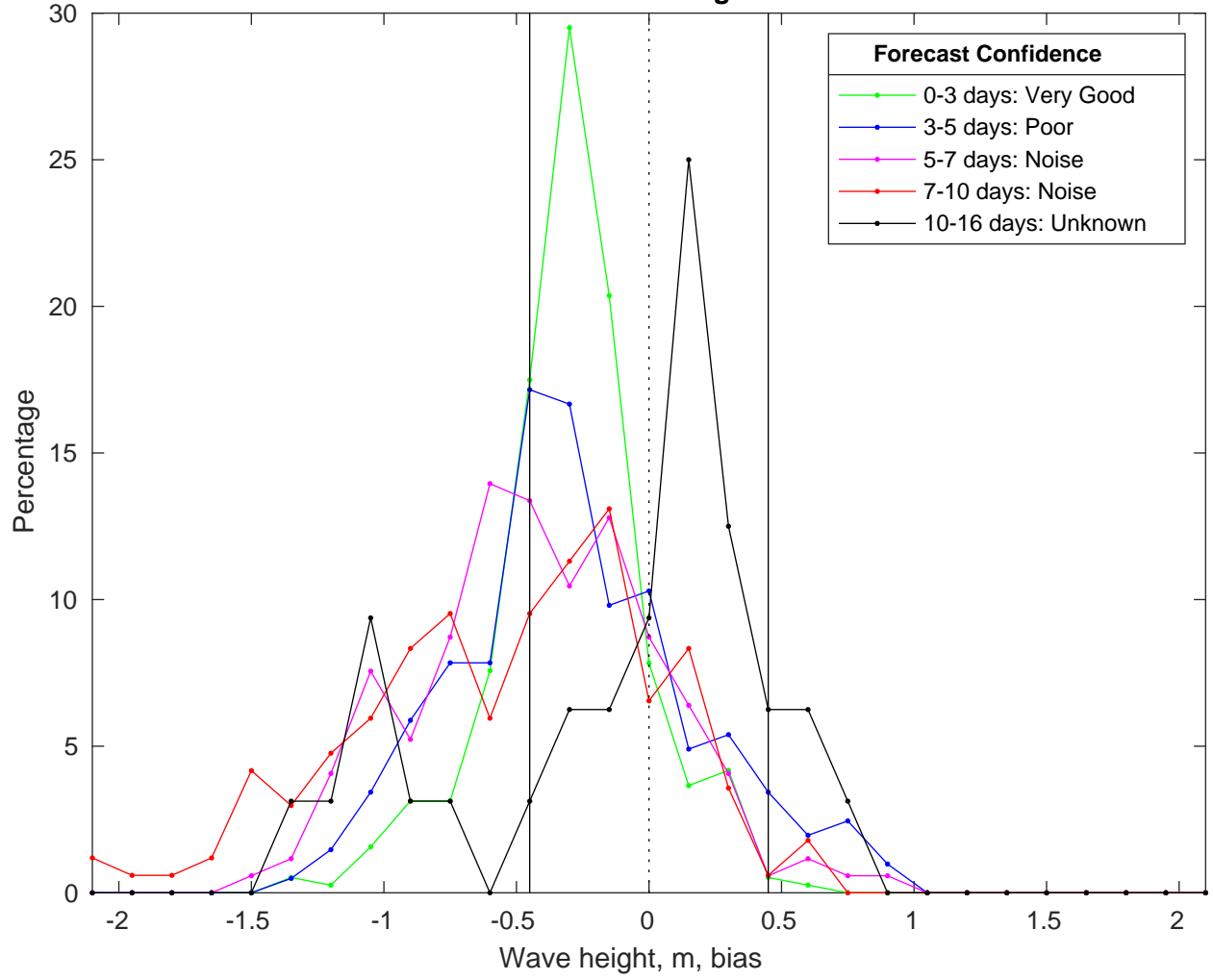
NDBC 46028 vs GFS Waves Bias Histogram: 12-Feb-2025
