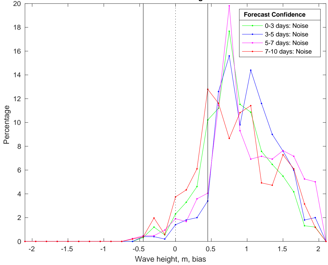
NDBC 46053 vs CMEMS Waves Bias Histogram: 12-Feb-2025
