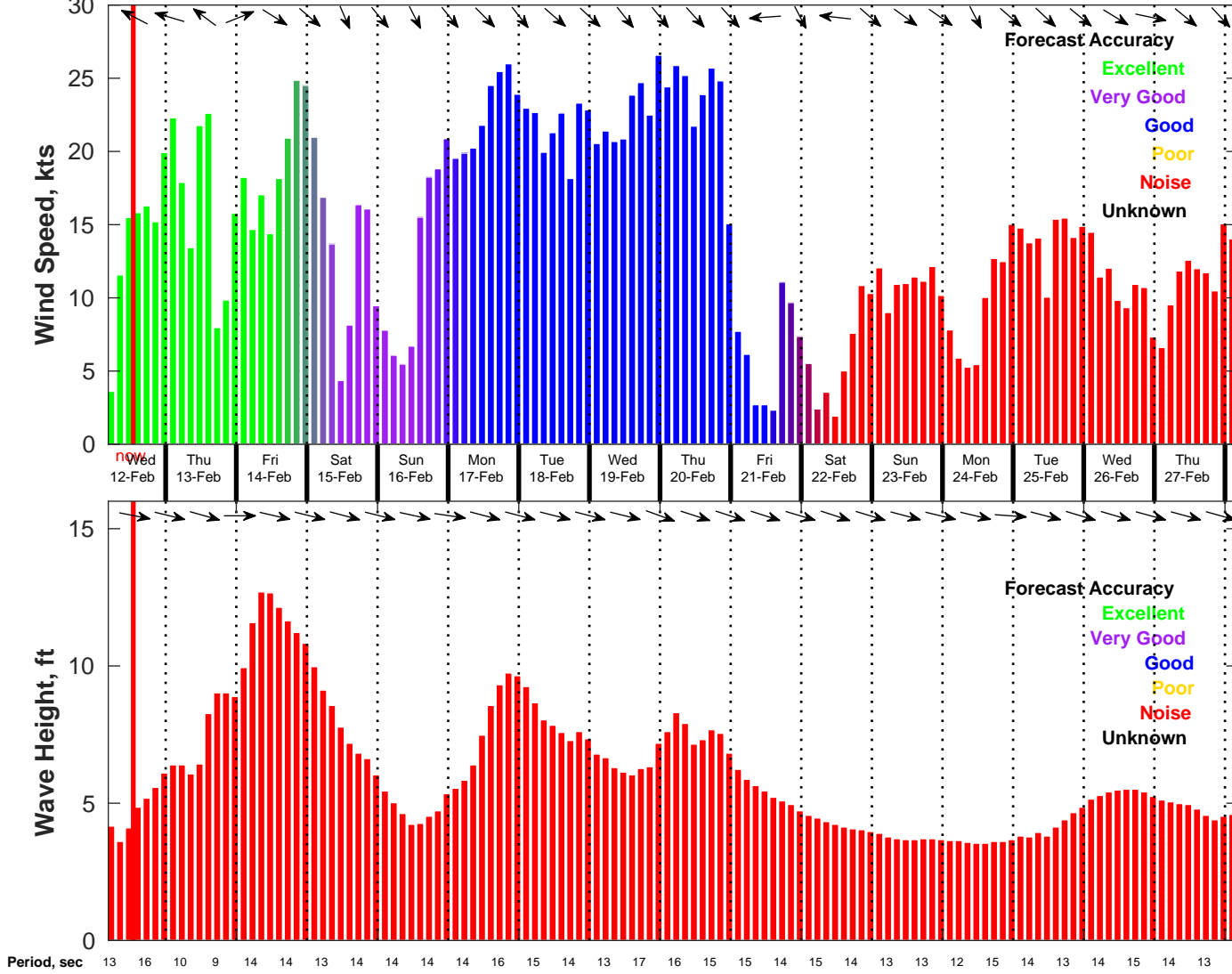
Wind & Wave Forecast for NDBC 46054 from 12-Feb-2025 04:00:00 to 28-Feb-2025 04:00:00
