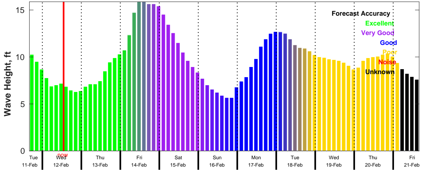
CMEMS Wave Forecast for NDBC 46069 from 11-Feb-2025 16:00:00 to 21-Feb-2025 16:00:00
