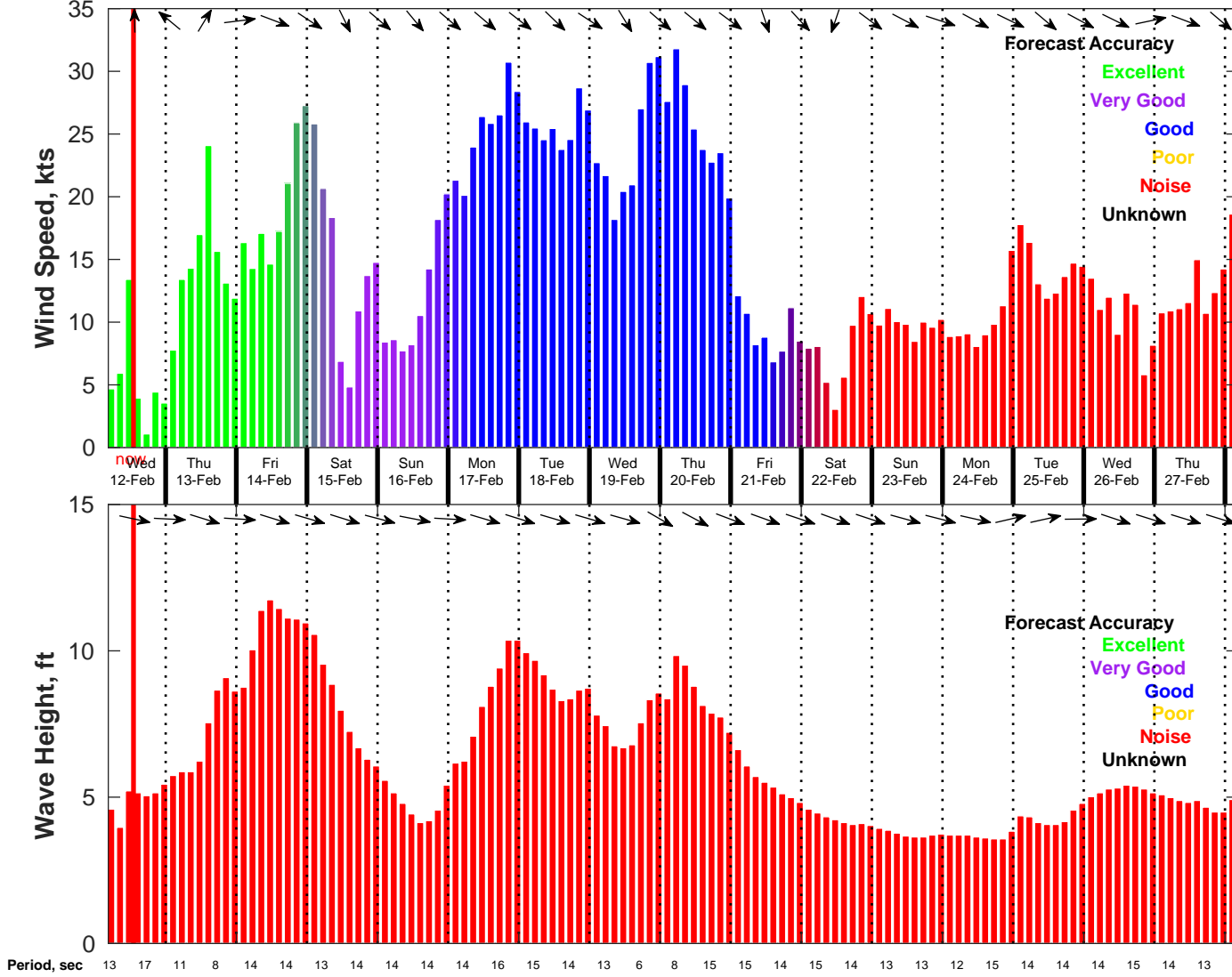
Wind & Wave Forecast for NDBC 46069 from 12-Feb-2025 04:00:00 to 28-Feb-2025 04:00:00
