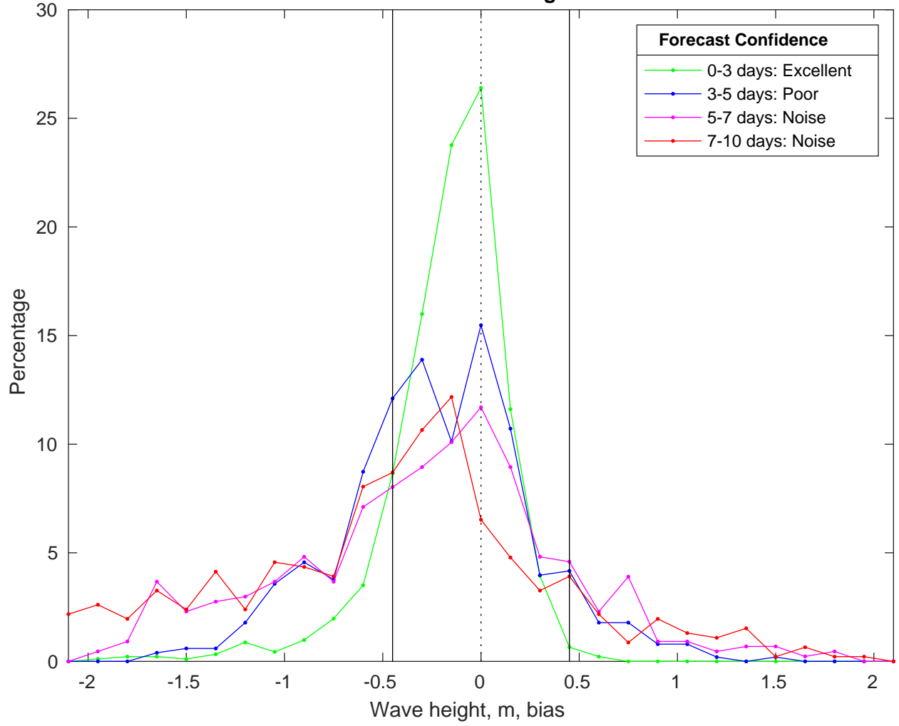
NDBC 46246 vs CMEMS Waves Bias Histogram: 12-Feb-2025
