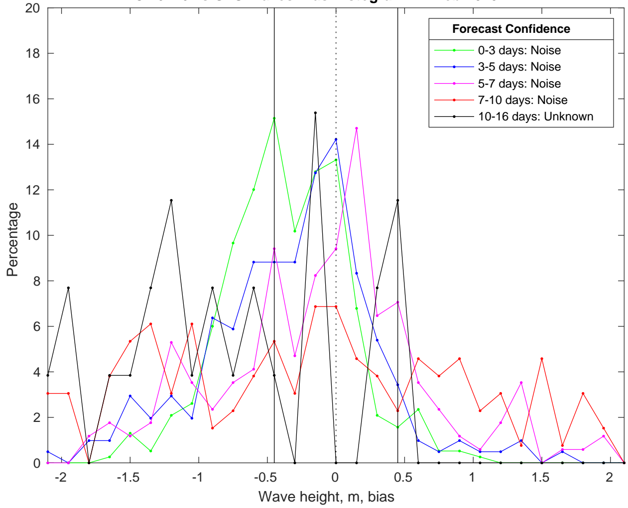
NDBC 46246 vs GFS Waves Bias Histogram: 12-Feb-2025
