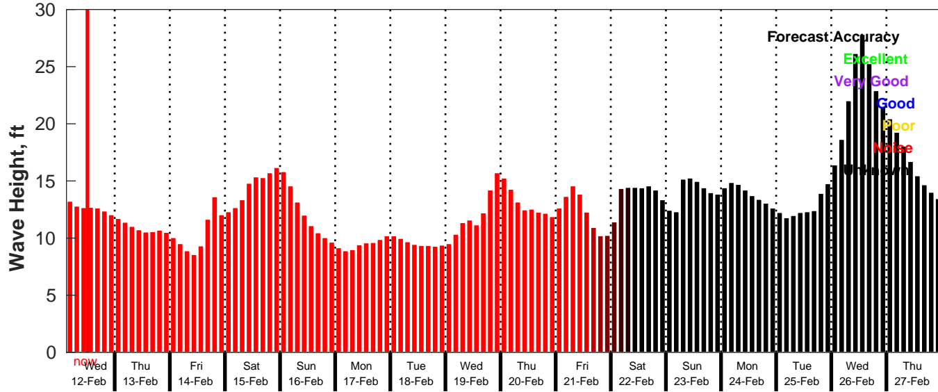
GFS Wave Forecast for NDBC 46246 from 12-Feb-2025 03:00:00 to 28-Feb-2025 03:00:00
