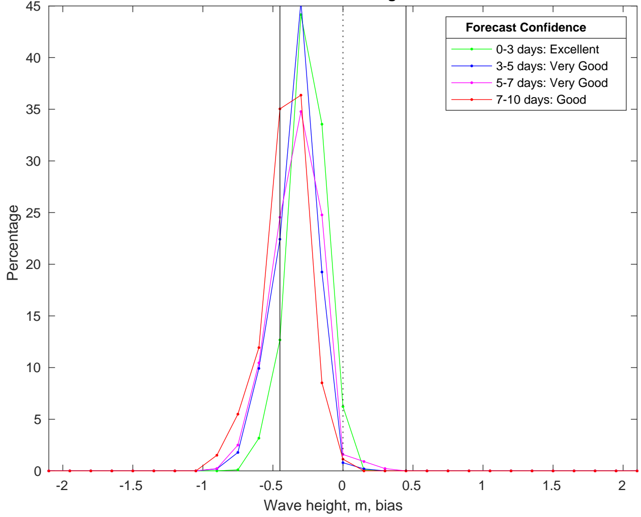
NDBC 51209 vs CMEMS Waves Bias Histogram: 12-Feb-2025
