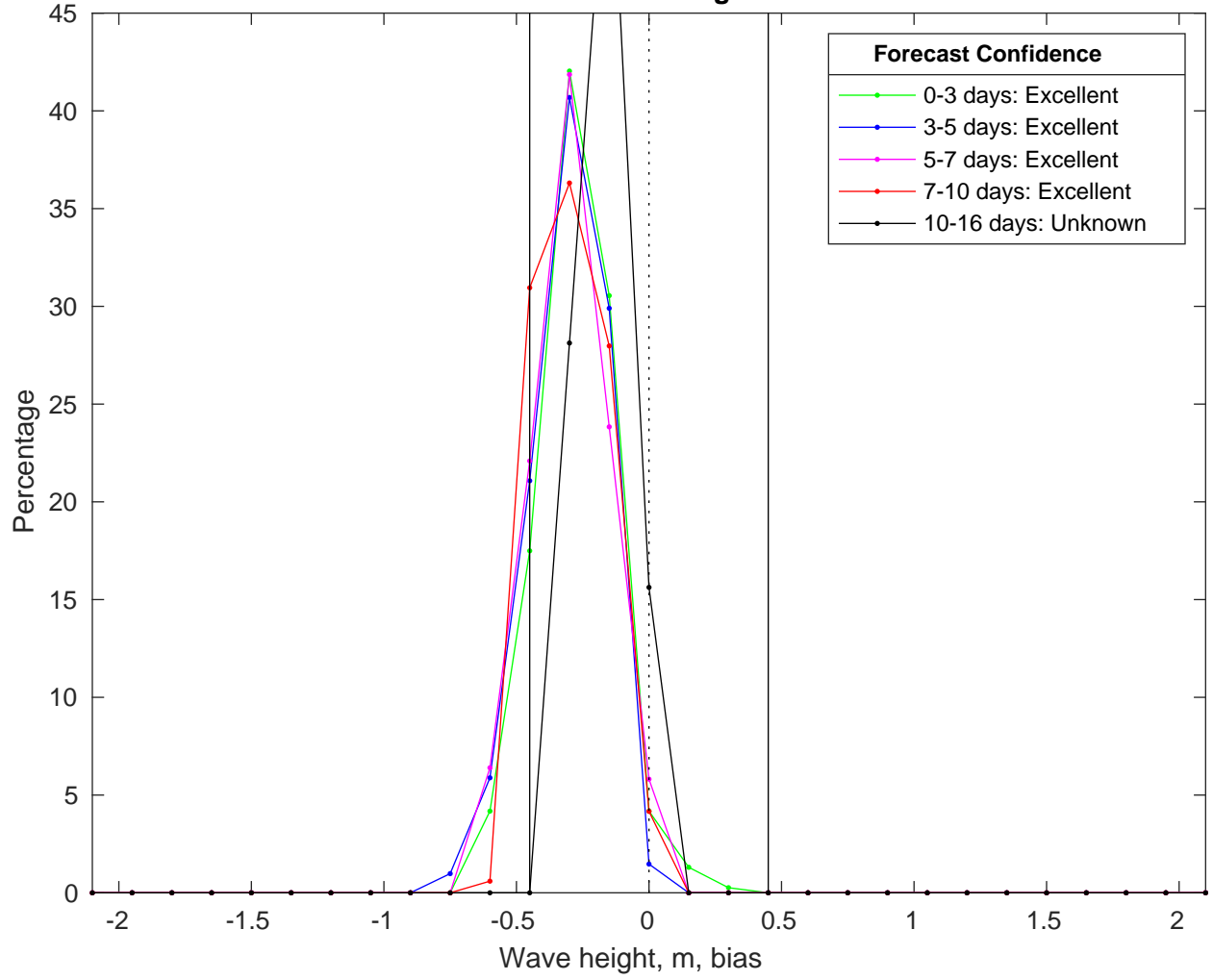
NDBC 51209 vs GFS Waves Bias Histogram: 12-Feb-2025
