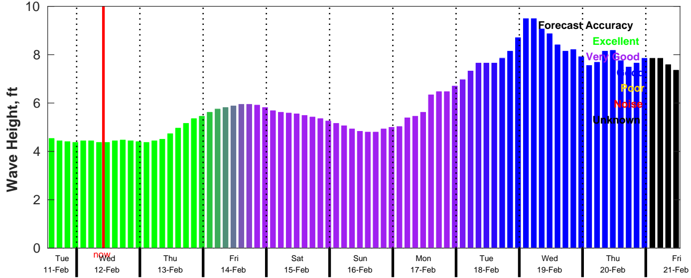
CMEMS Wave Forecast for NDBC 51209 from 11-Feb-2025 13:00:00 to 21-Feb-2025 13:00:00
