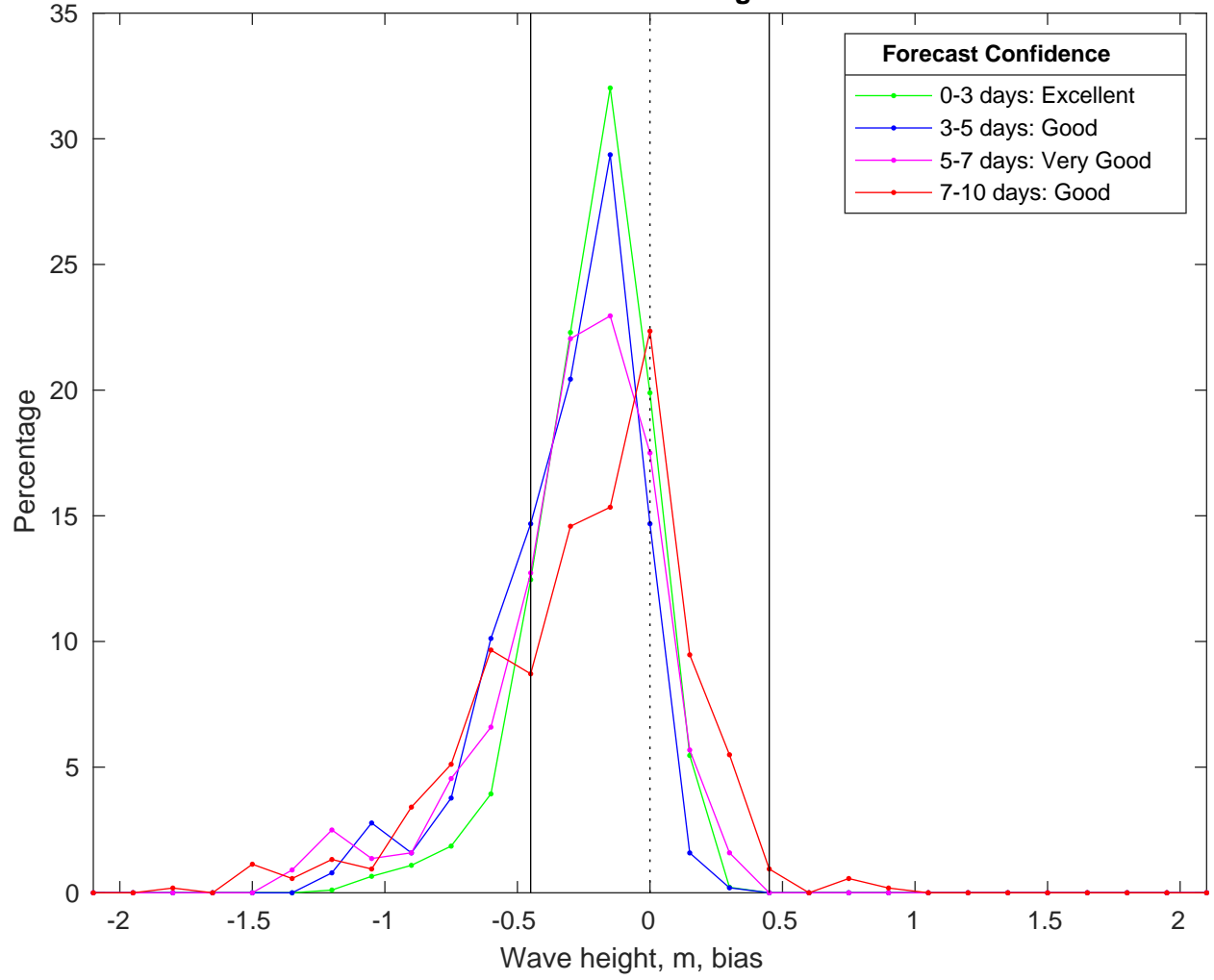
NDBC 52211 vs CMEMS Waves Bias Histogram: 12-Feb-2025
