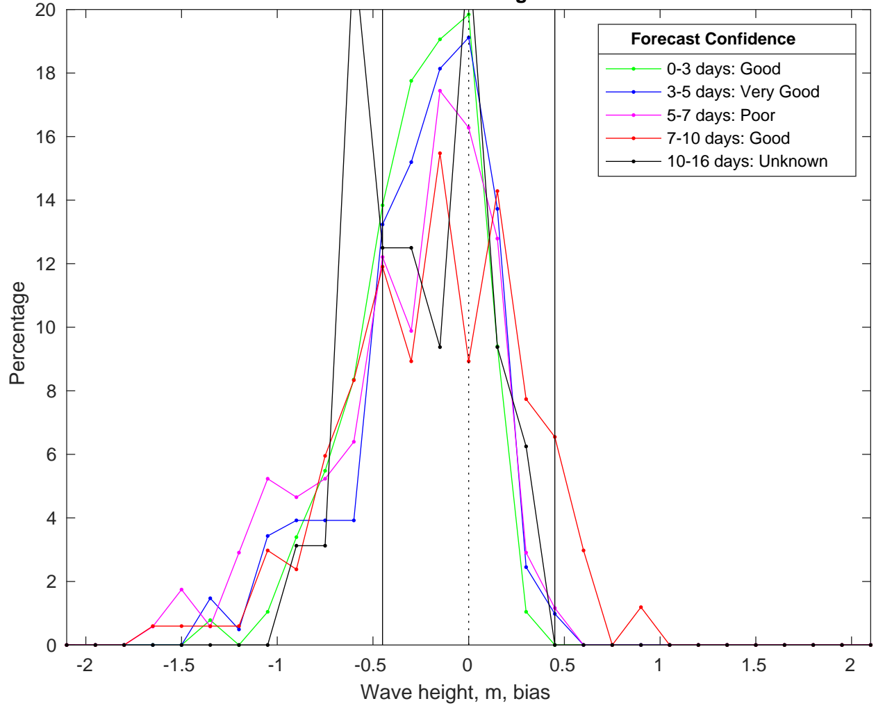
NDBC 52211 vs GFS Waves Bias Histogram: 12-Feb-2025
