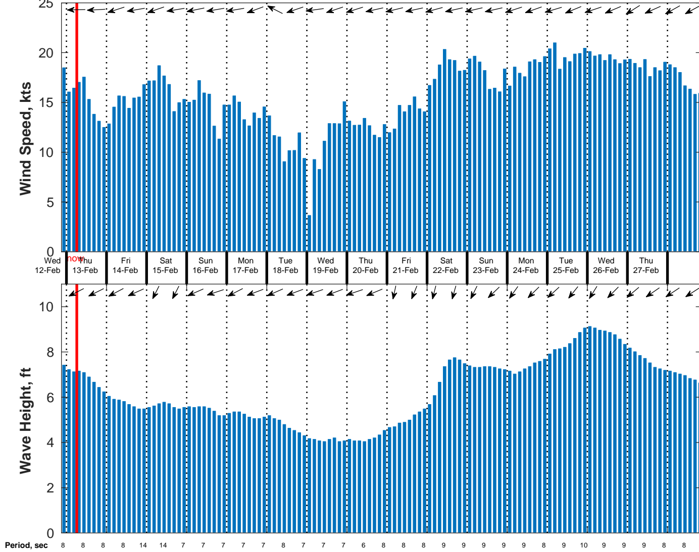
Wind & Wave Forecast for NDBC 52212 from 12-Feb-2025 21:00:00 to 28-Feb-2025 21:00:00
