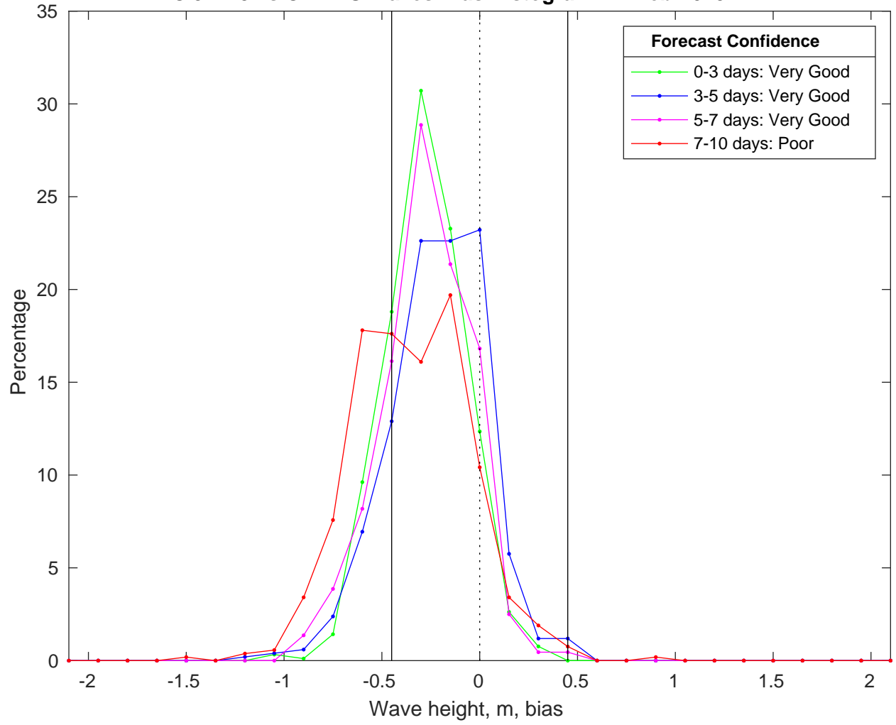
NDBC 52213 vs CMEMS Waves Bias Histogram: 12-Feb-2025
