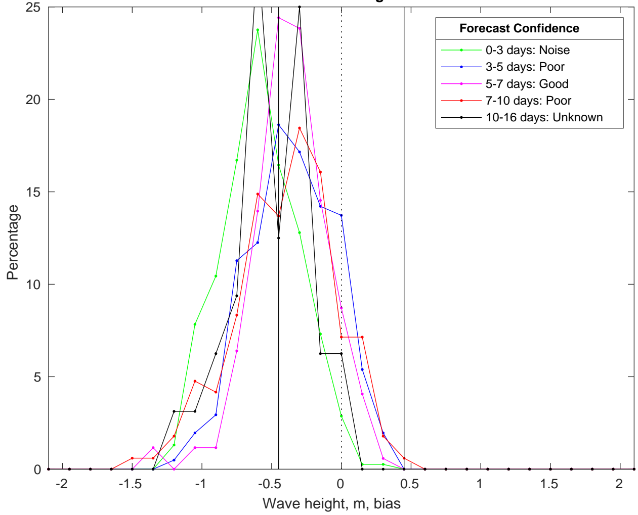
NDBC 52213 vs GFS Waves Bias Histogram: 12-Feb-2025
