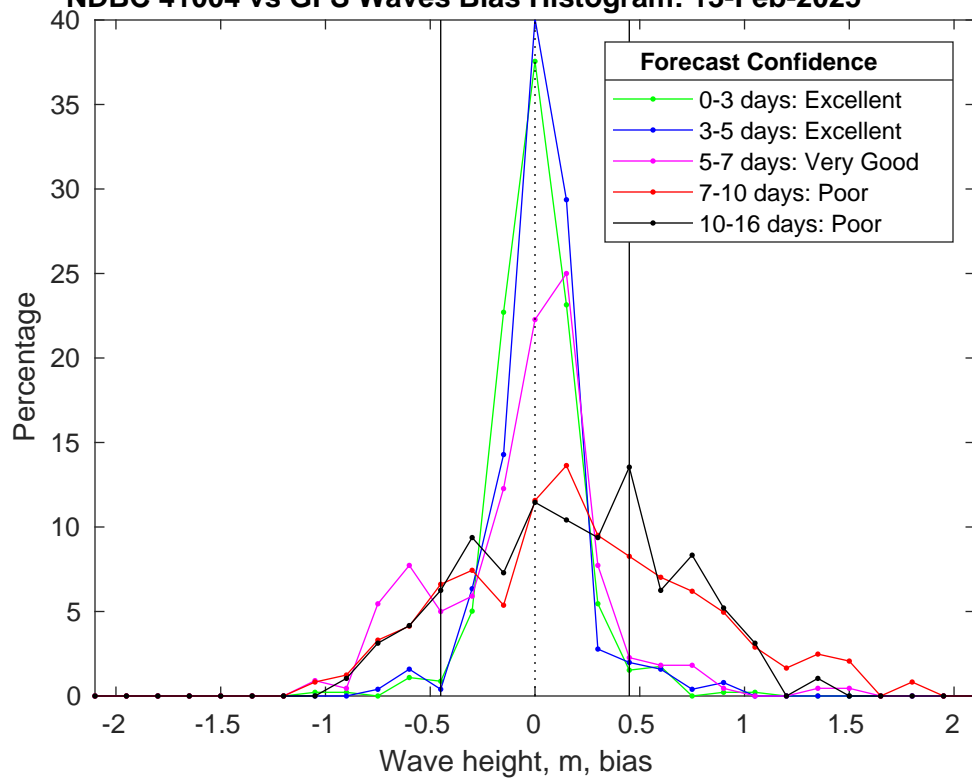
NDBC 41004 vs GFS Waves Bias Histogram: 13-Feb-2025
