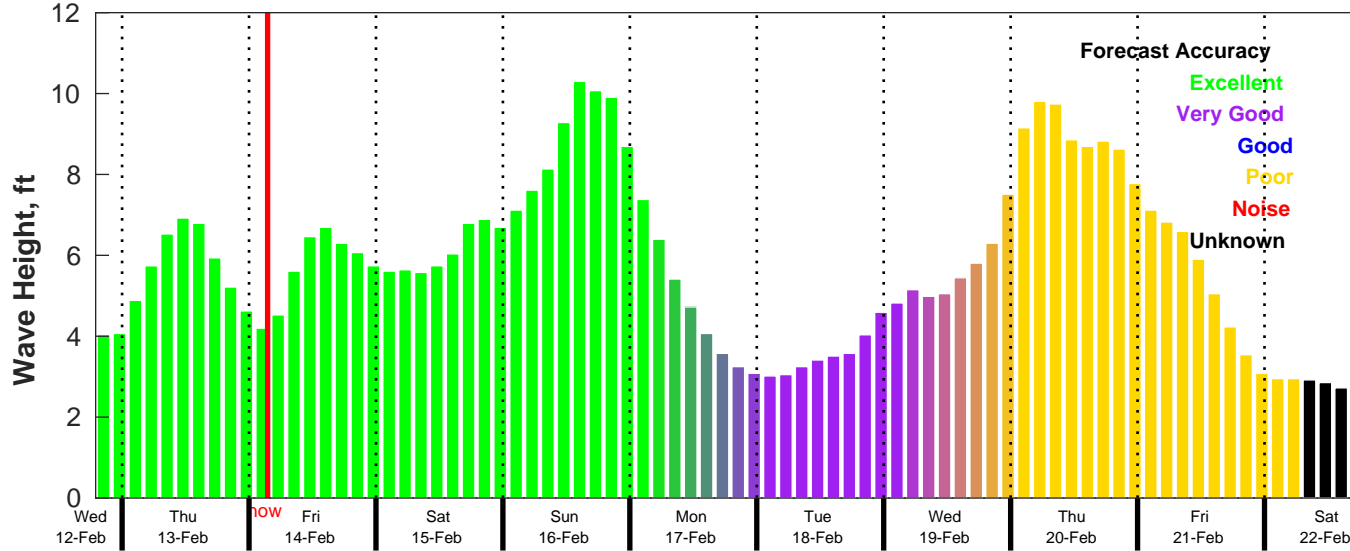
CMEMS Wave Forecast for NDBC 41004 from 12-Feb-2025 19:00:00 to 22-Feb-2025 19:00:00
