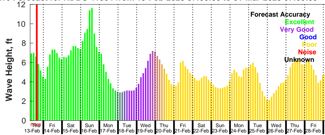
GFS Wave Forecast for NDBC 41004 from 13-Feb-2025 07:00:00 to 01-Mar-2025 07:00:00
