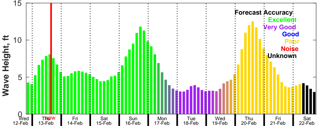
CMEMS Wave Forecast for NDBC 41013 from 12-Feb-2025 19:00:00 to 22-Feb-2025 19:00:00
