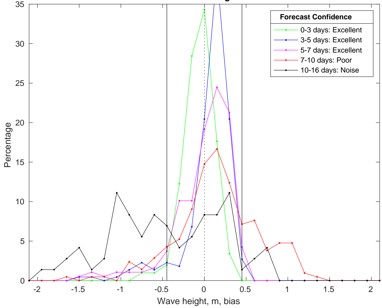
NDBC 42019 vs GFS Waves Bias Histogram: 13-Feb-2025
