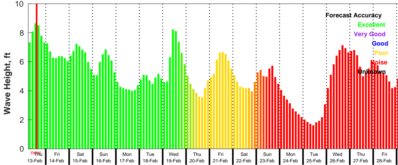
GFS Wave Forecast for NDBC 42019 from 13-Feb-2025 06:00:00 to 01-Mar-2025 06:00:00
