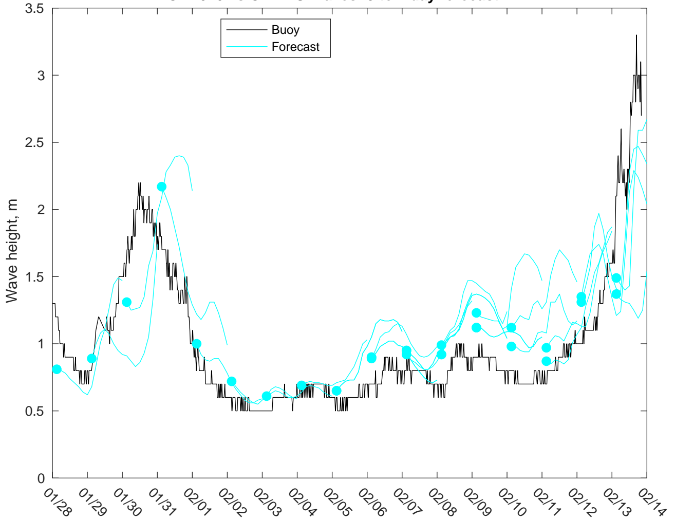
NDBC 42020 vs CMEMS Waves: 5 to 7 day forecast
