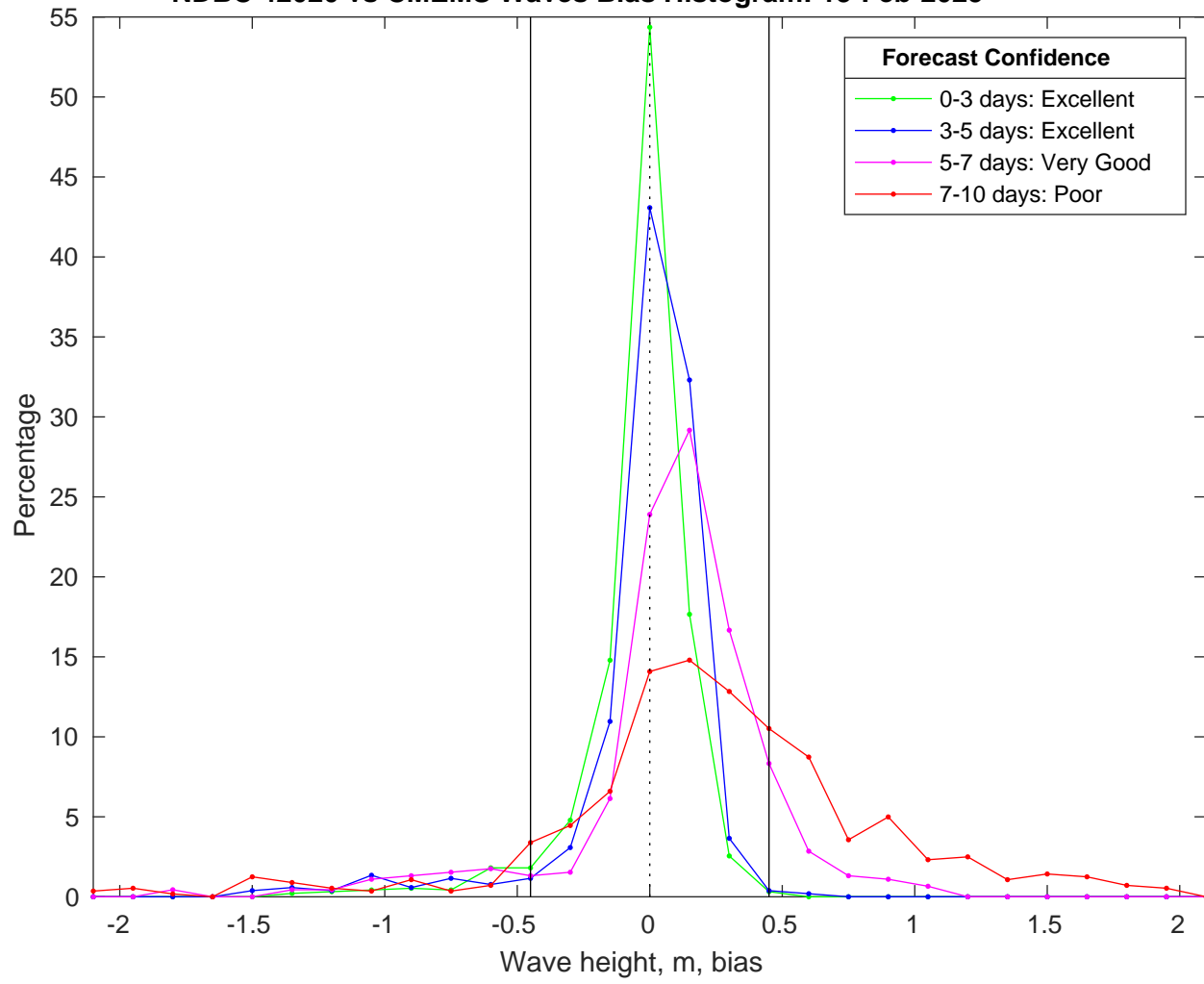
NDBC 42020 vs CMEMS Waves Bias Histogram: 13-Feb-2025
