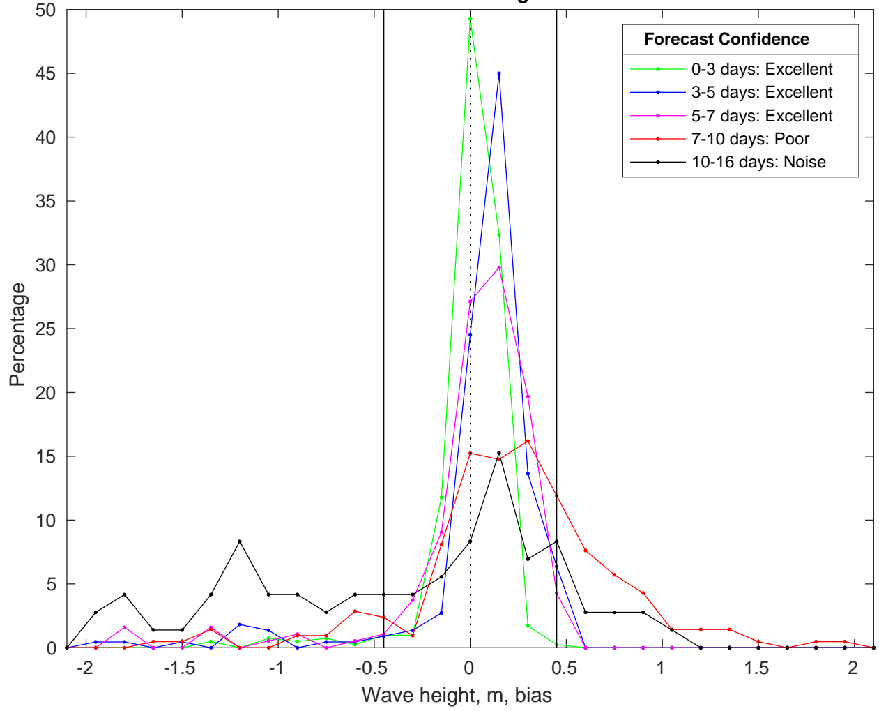
NDBC 42020 vs GFS Waves Bias Histogram: 13-Feb-2025
