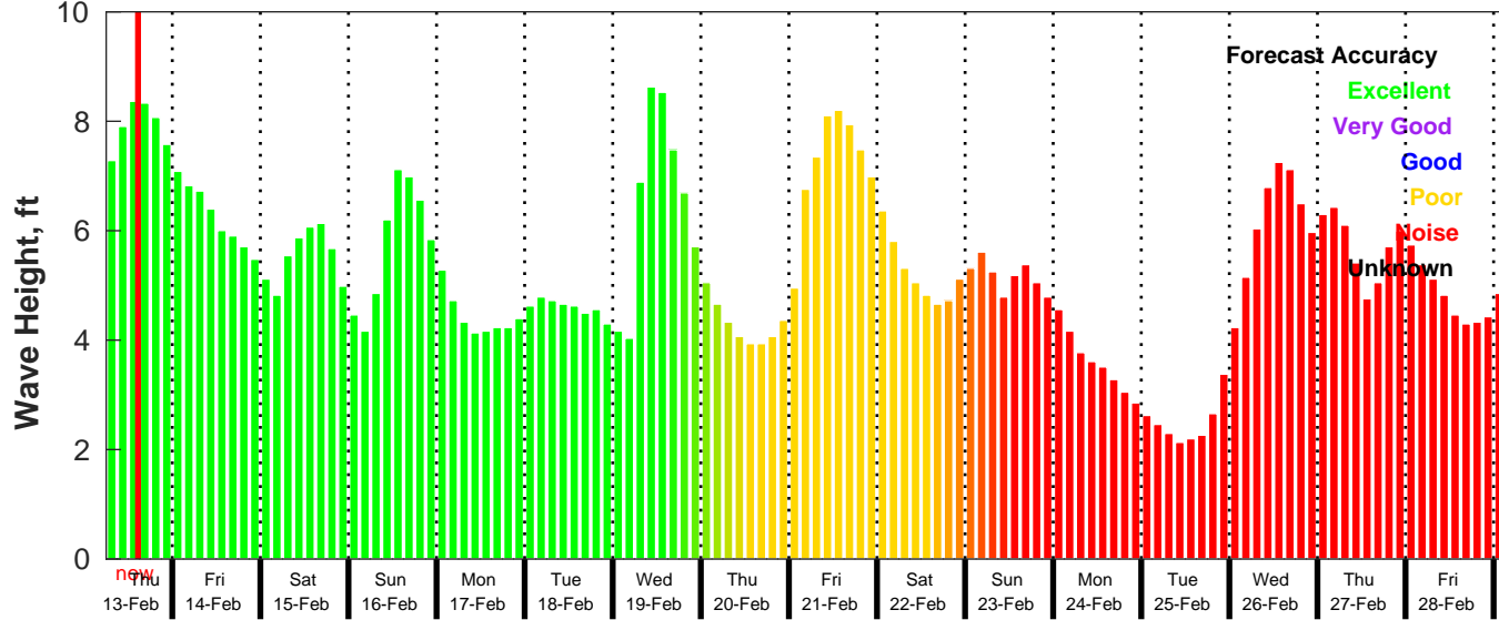
GFS Wave Forecast for NDBC 42020 from 13-Feb-2025 06:00:00 to 01-Mar-2025 06:00:00
