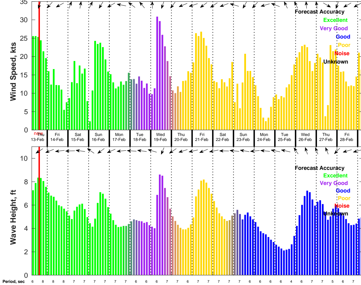
Wind & Wave Forecast for NDBC 42020 from 13-Feb-2025 06:00:00 to 01-Mar-2025 06:00:00
