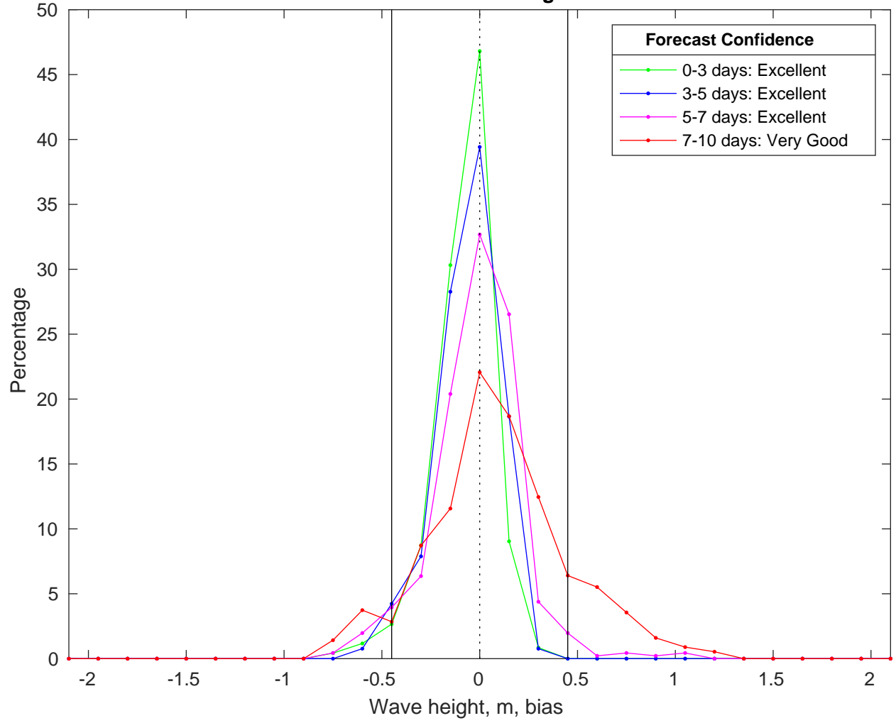
NDBC 42035 vs CMEMS Waves Bias Histogram: 13-Feb-2025
