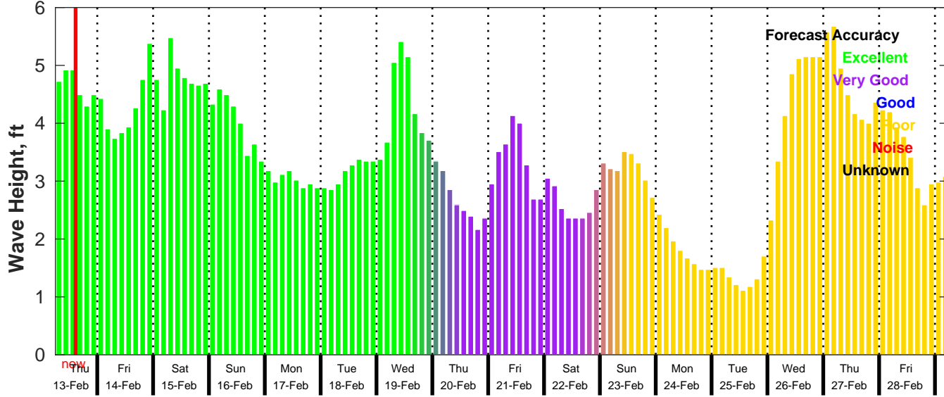
GFS Wave Forecast for NDBC 42035 from 13-Feb-2025 06:00:00 to 01-Mar-2025 06:00:00
