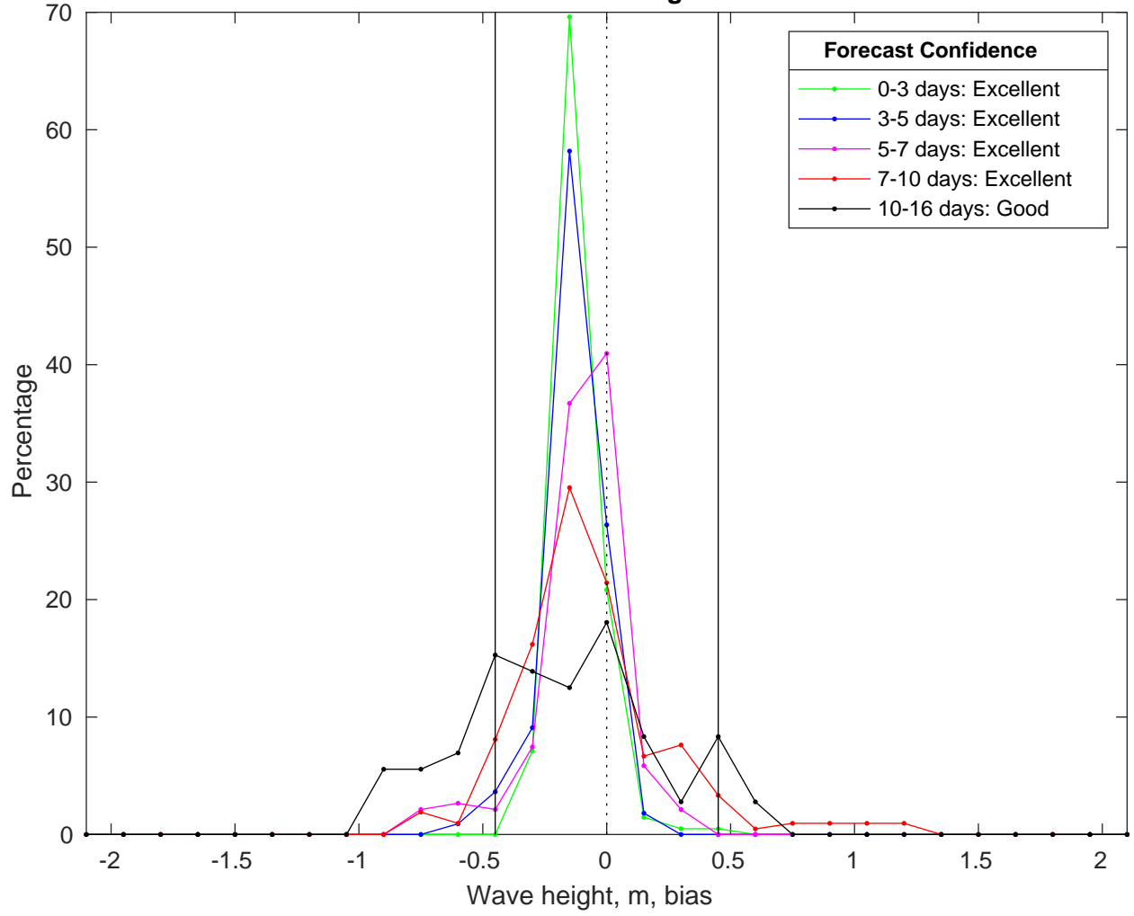
NDBC 42036 vs GFS Waves Bias Histogram: 13-Feb-2025
