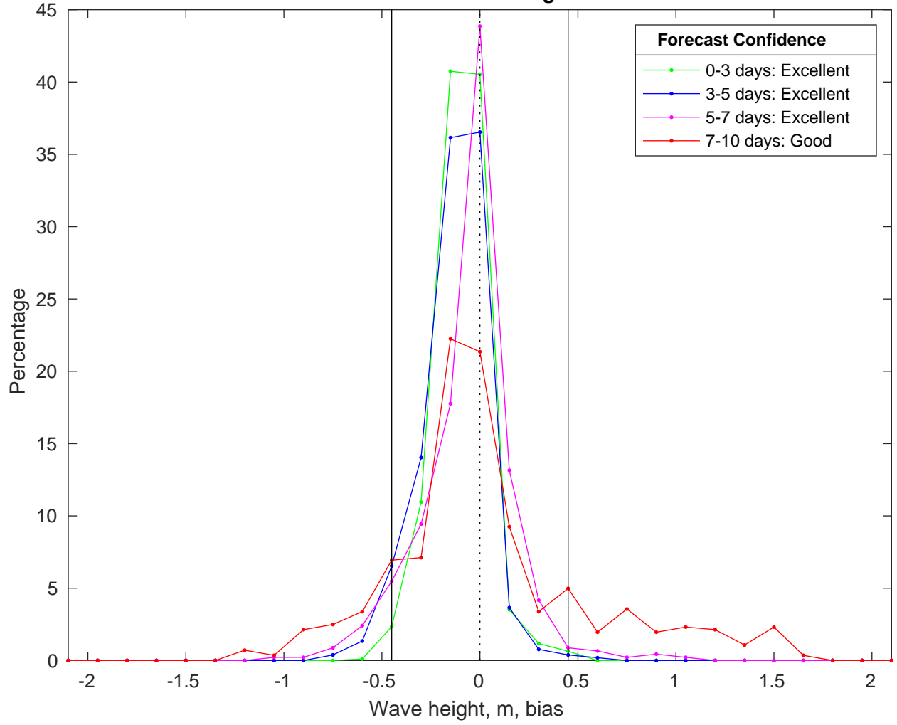
NDBC 42040 vs CMEMS Waves Bias Histogram: 13-Feb-2025
