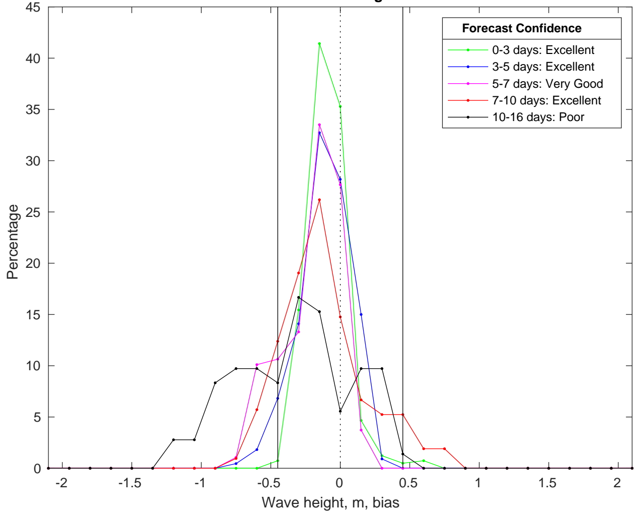
NDBC 42040 vs GFS Waves Bias Histogram: 13-Feb-2025
