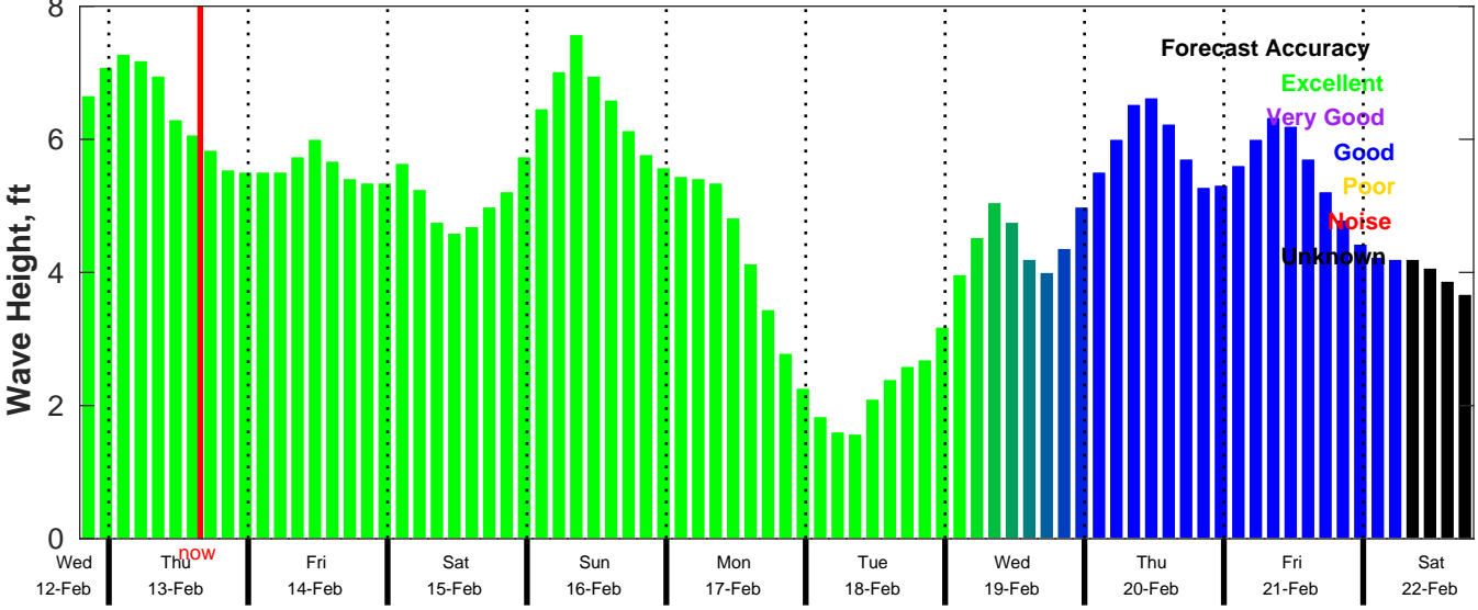
CMEMS Wave Forecast for NDBC 42040 from 12-Feb-2025 19:00:00 to 22-Feb-2025 19:00:00
