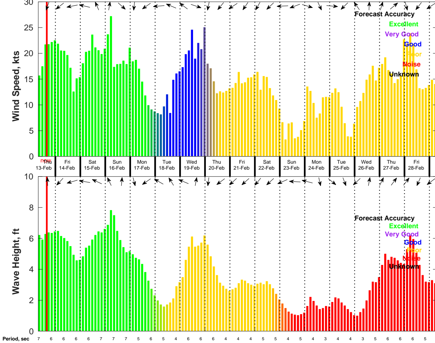
Wind & Wave Forecast for NDBC 42040 from 13-Feb-2025 07:00:00 to 01-Mar-2025 07:00:00
