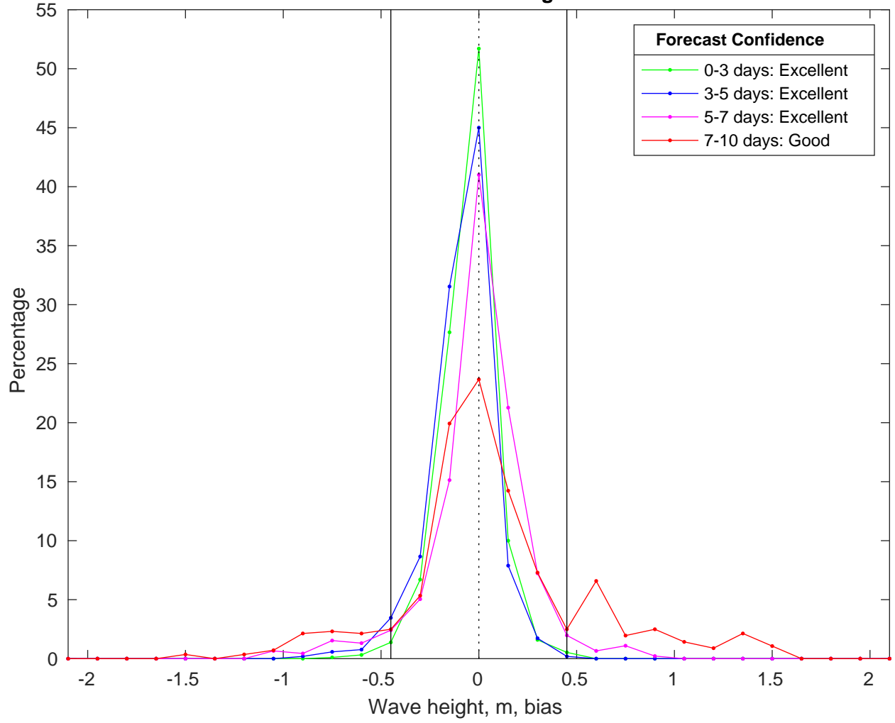
NDBC 42084 vs CMEMS Waves Bias Histogram: 13-Feb-2025
