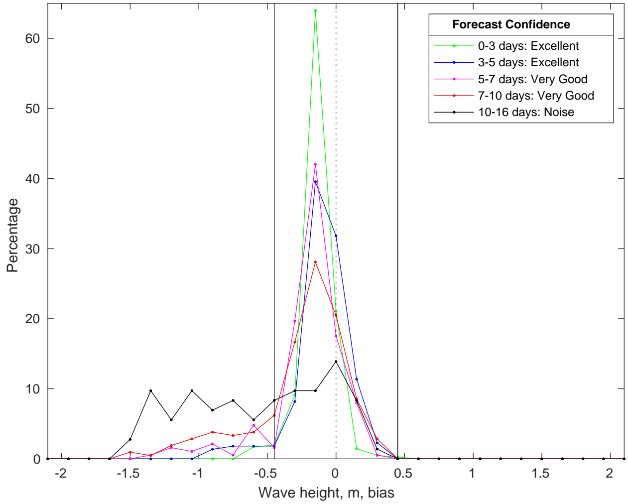
NDBC 42084 vs GFS Waves Bias Histogram: 13-Feb-2025
