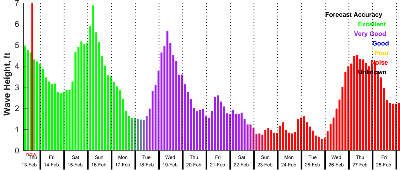
GFS Wave Forecast for NDBC 42084 from 13-Feb-2025 07:00:00 to 01-Mar-2025 07:00:00
